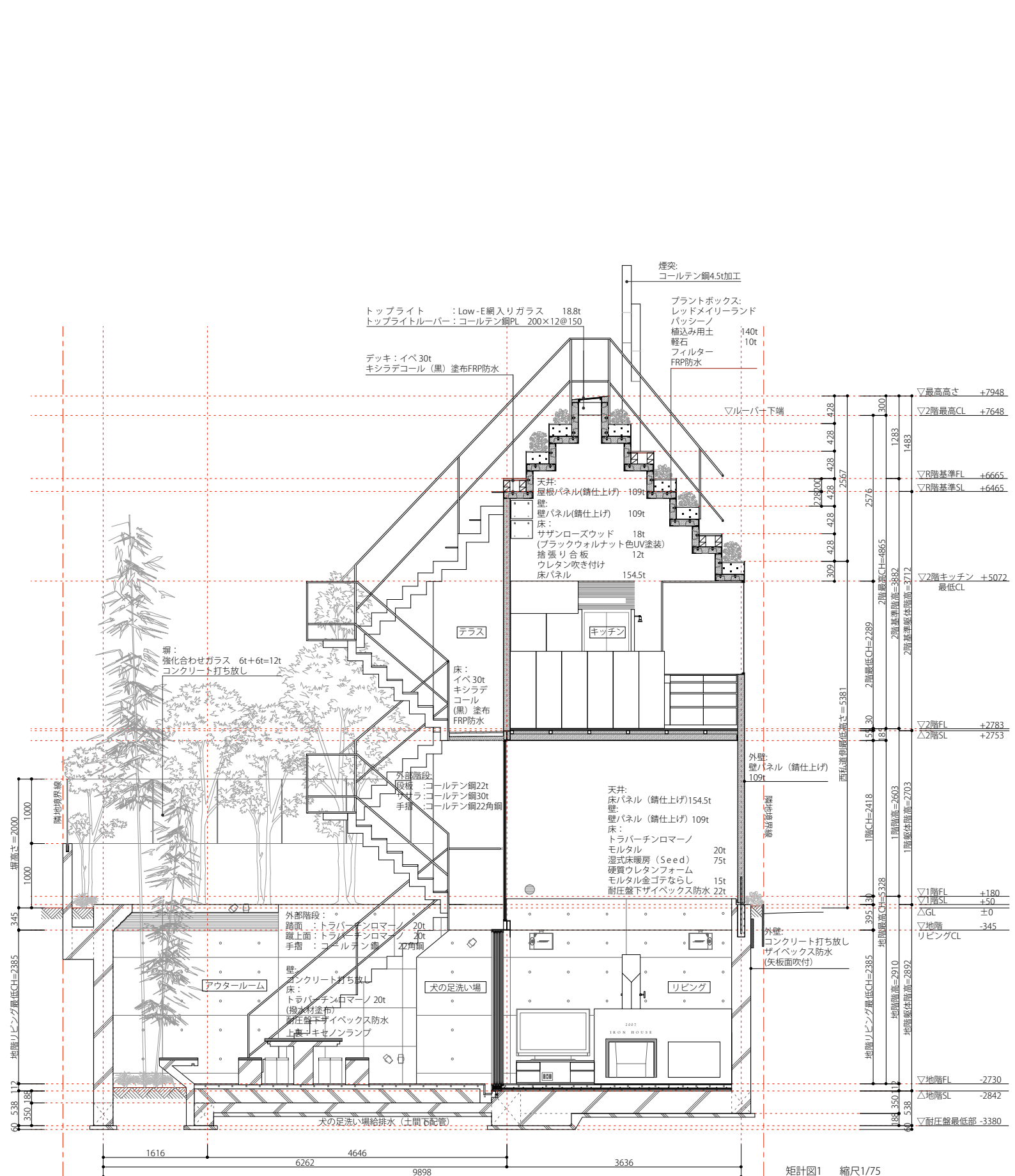
矩計図1 縮尺1/75
